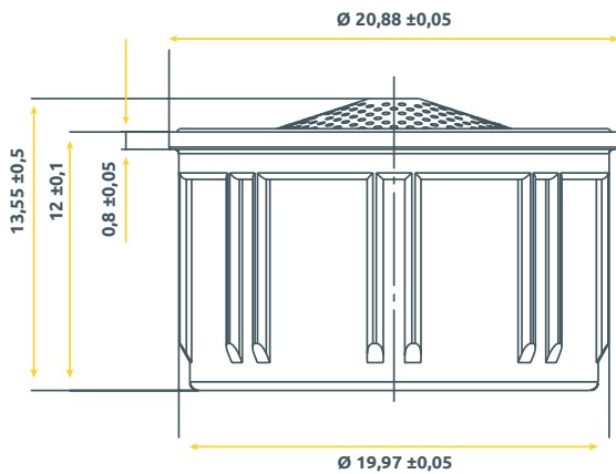
Atomizer-STD-IT Single Jet Dimensions are according to EN246
